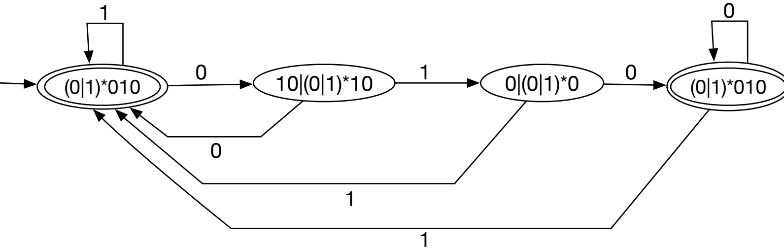
(e) (0|1)^*010
