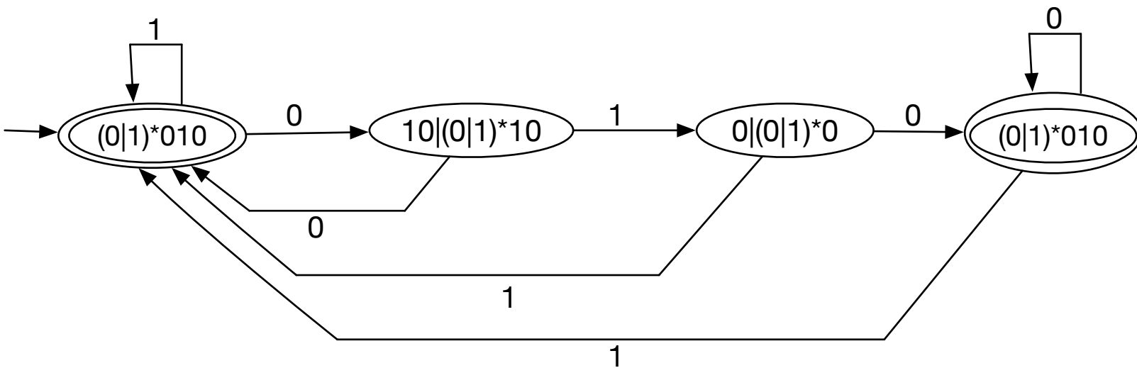
(e) (0|1)^*010
