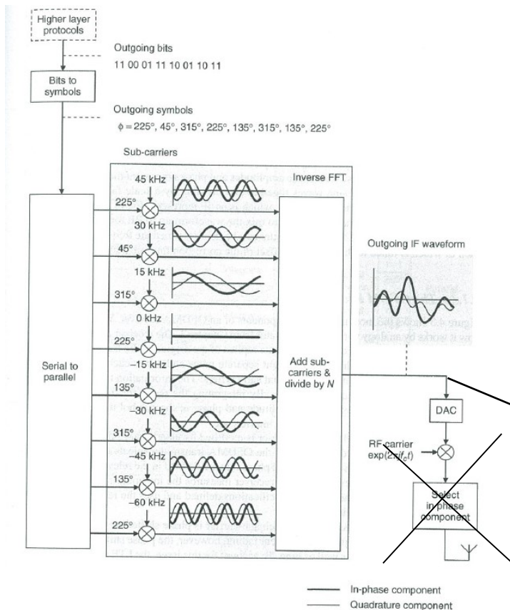
Figure 4.2 Processing steps in an OFDM transmitter
