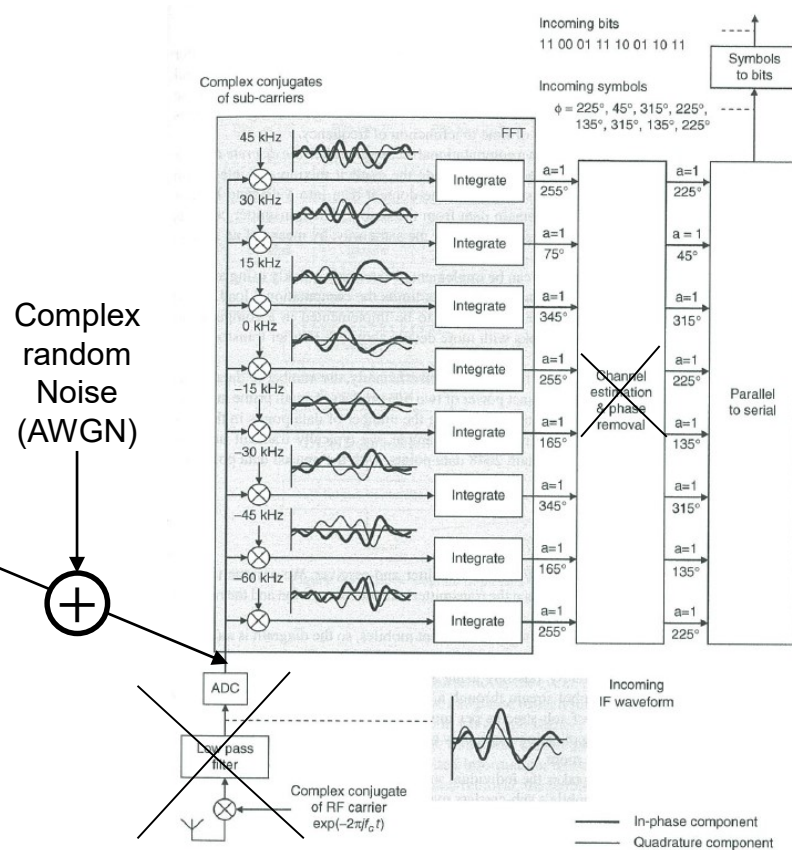
Figure 4.3 Processing steps in an OFDM receiver
